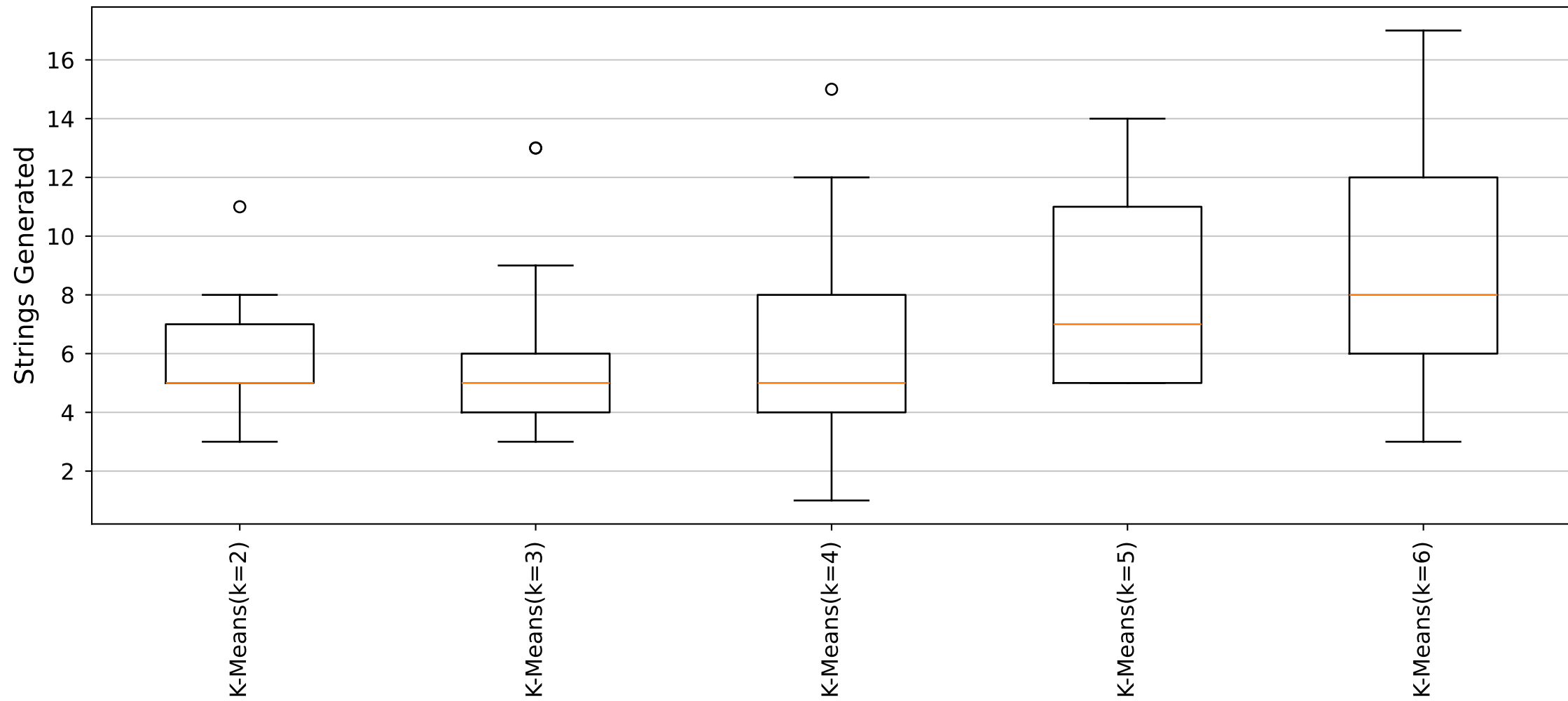
YARA Rules Strings Generated Distribution (Cluster18_Size6 dataset)
